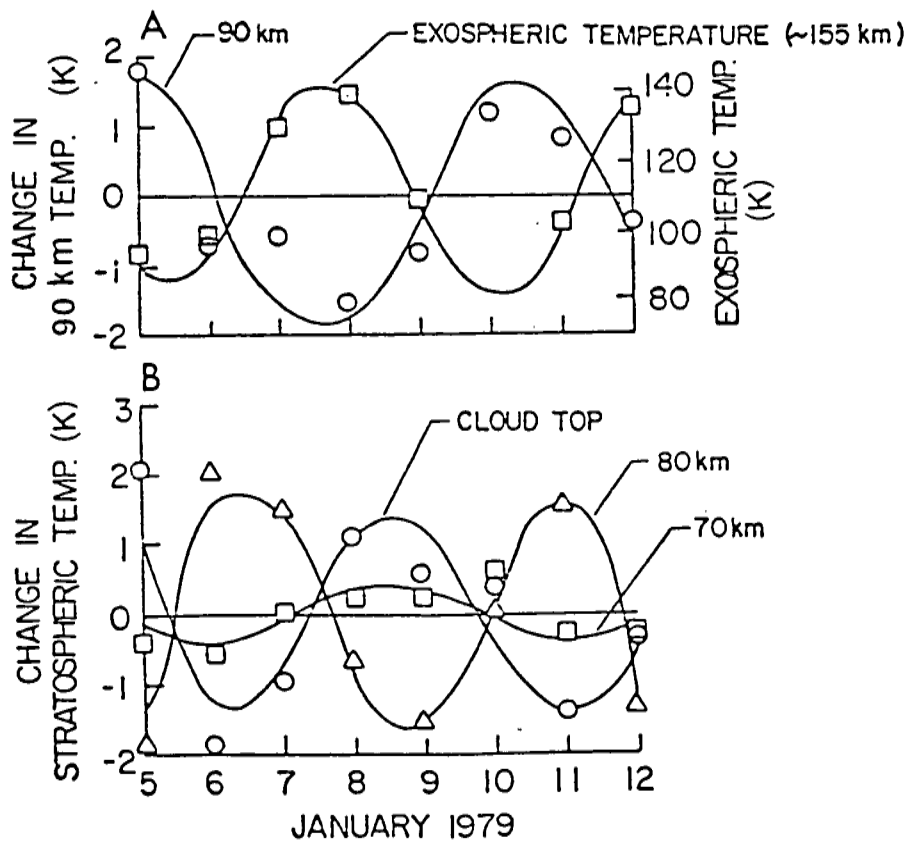
Figure 3.15. Inferred temperature variations at 90 km and 155 km (ref. 57).
