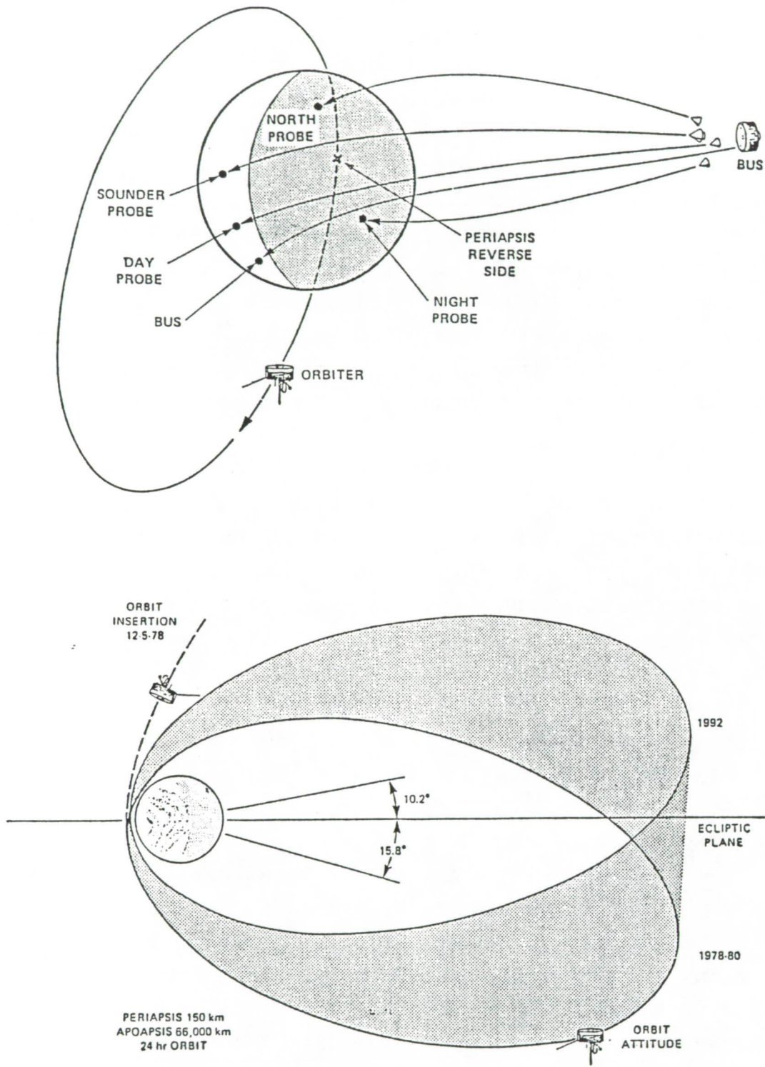
Figure 1.2. The Orbiter in position, the bus has released its probes (top) (ref. 2a). The orbit as it appeared in 1978-80 and as it will appear in 1992 (bottom) (ref. 2b).
