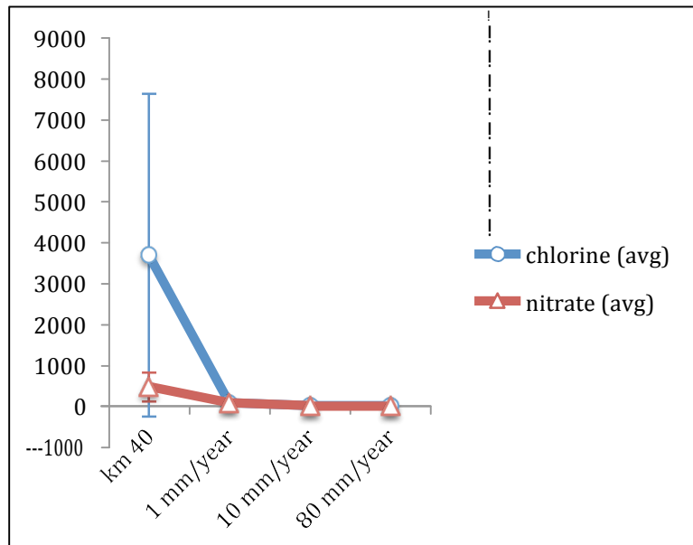
Figure 3 – Preliminary data from Figure 2, but also including data from km 40
