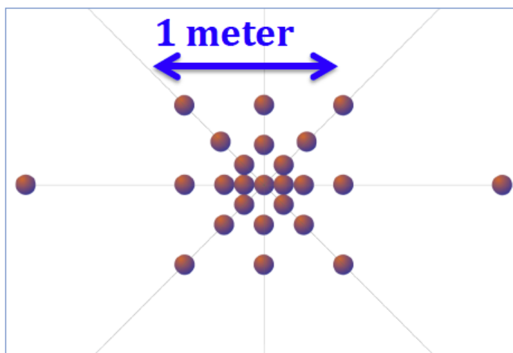
Figure 1 - Radial grid for our “horizontal” heterogeneity sampling!
