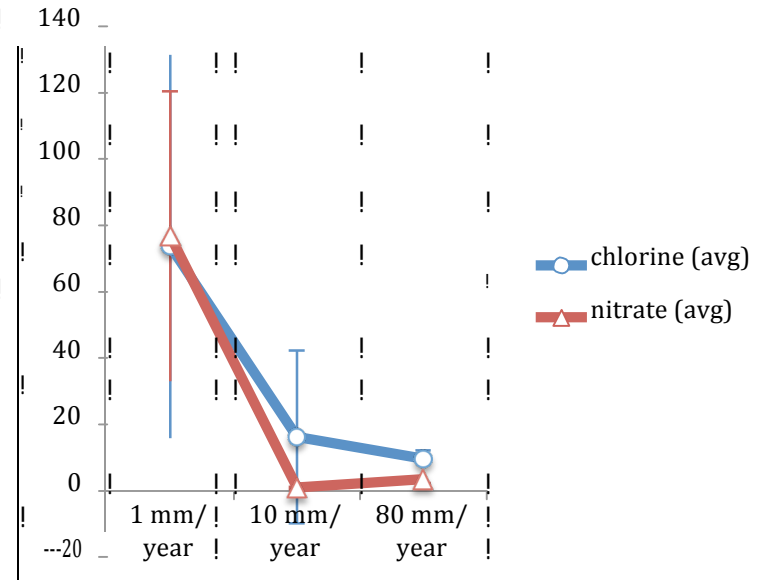
Figure 2 – Preliminary Data from our horizontal transect
